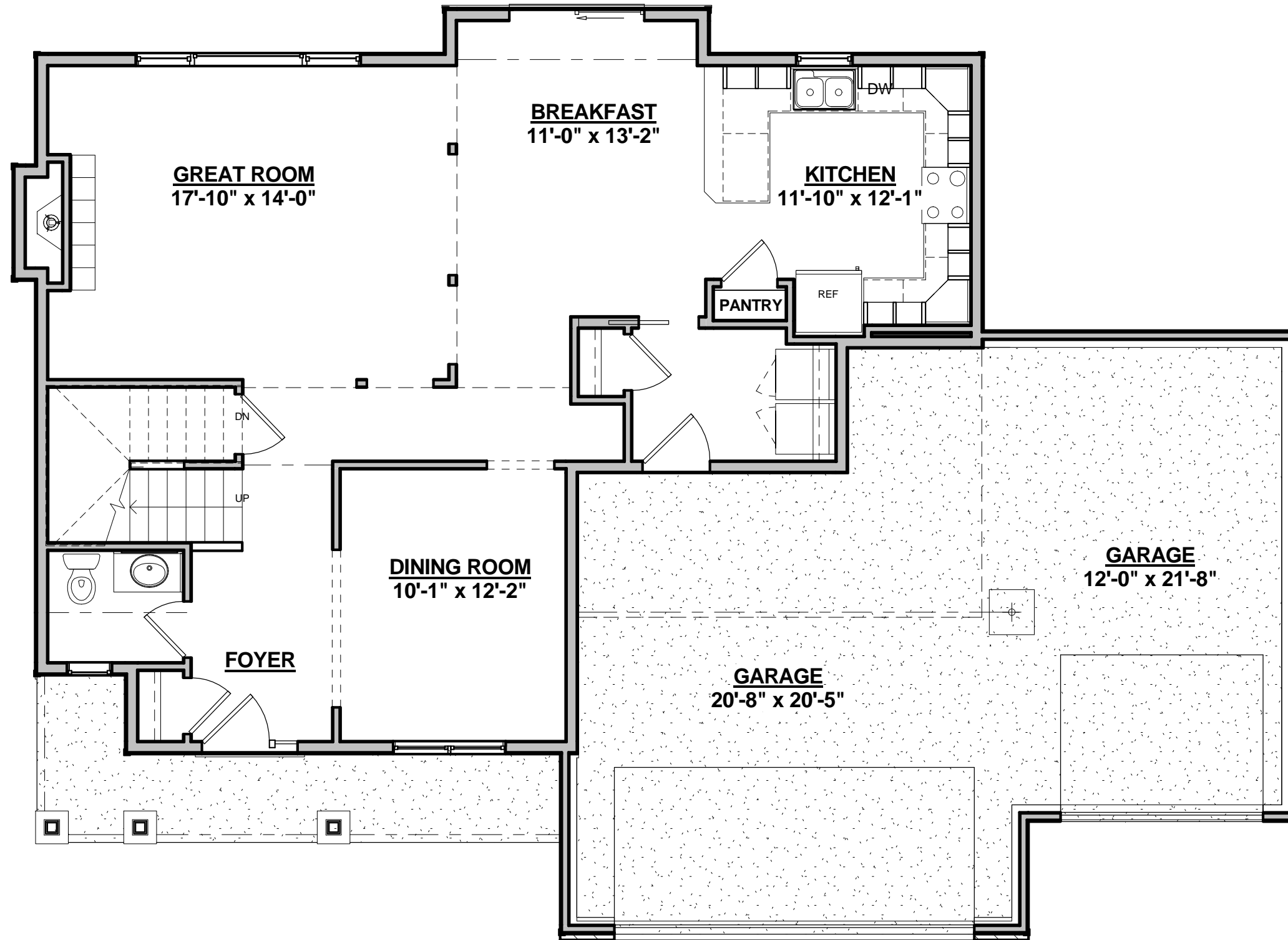
Sutton First Floor 2049 3/16" = 1'-0"
