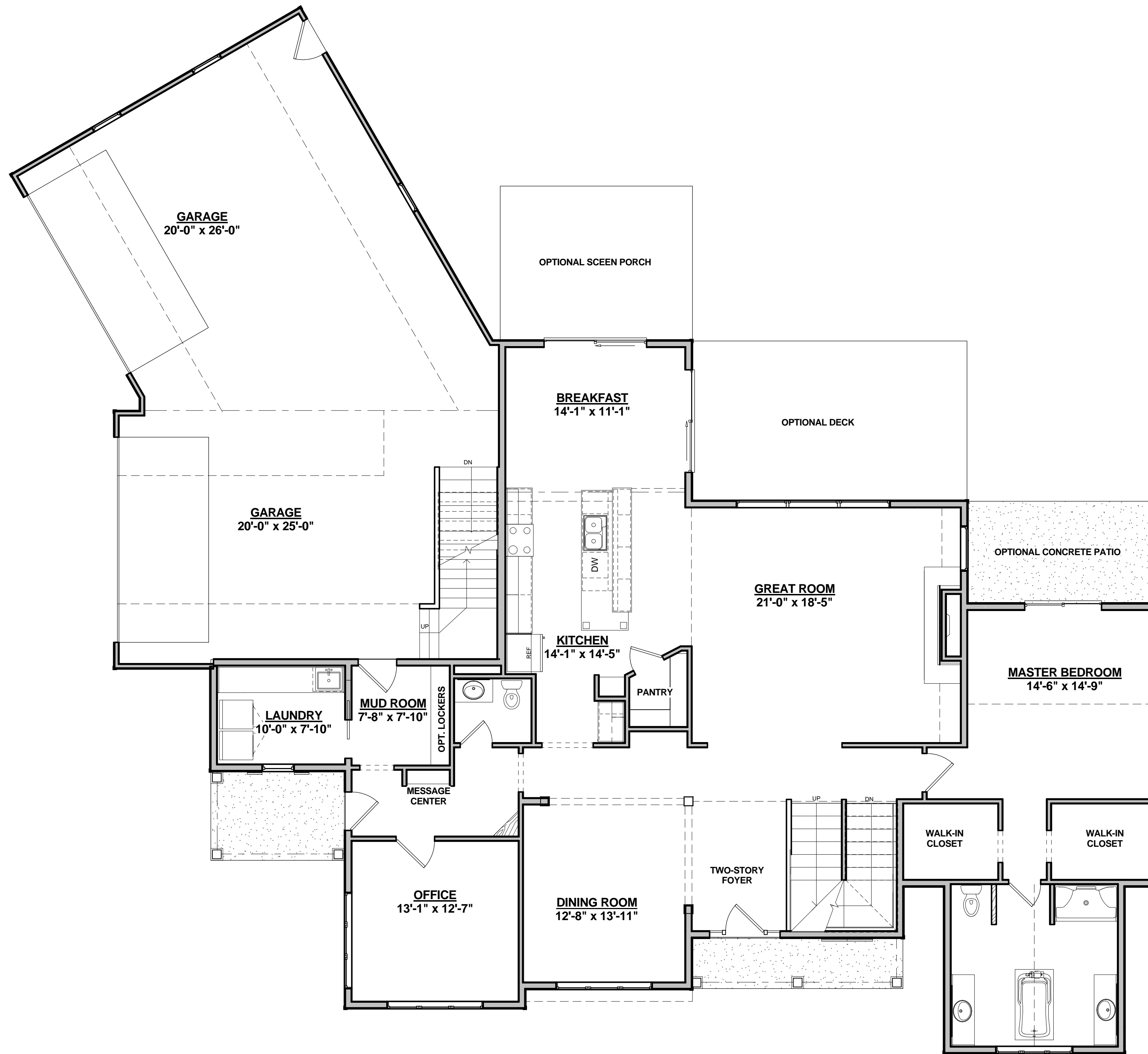
Prescott_First Floor_3445 3/16" = 1'-0"
