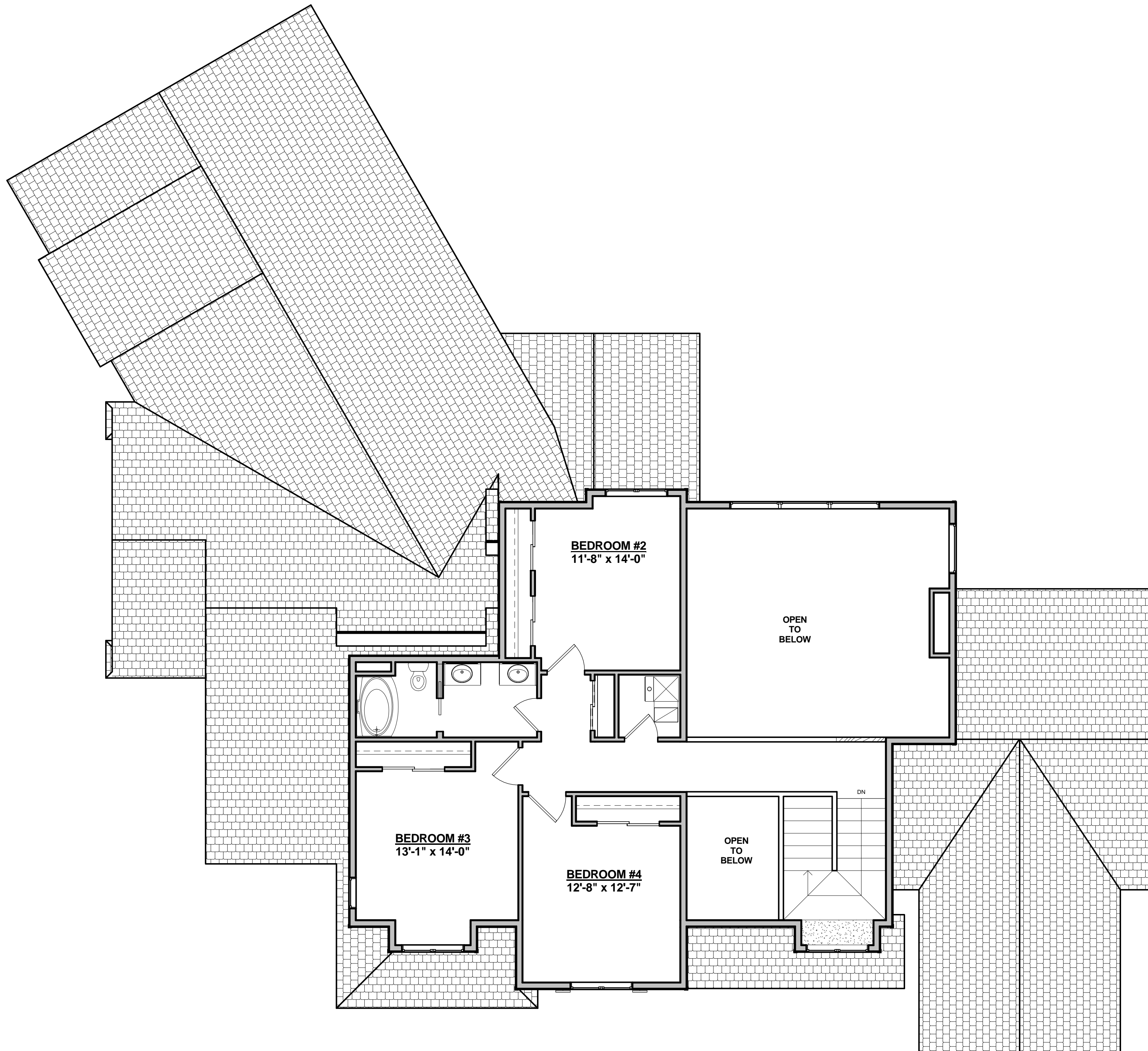
Prescott Second Floor 3445 3/16" = 1'-0"
